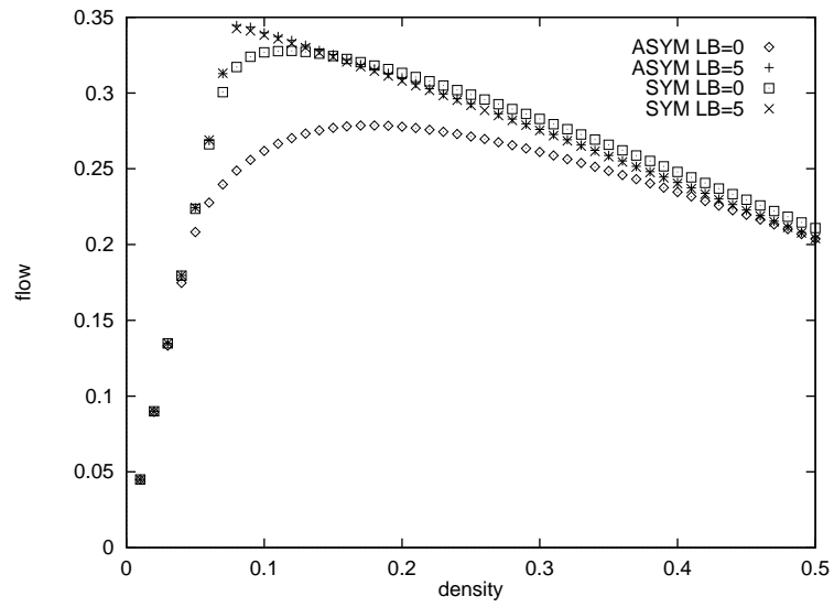
Figure 13: Flow\ p_{change} = 1.0 , different LookBack
