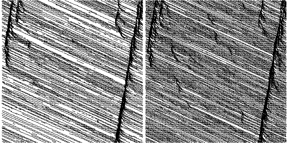
Figure 10: asymmetric, l_{o,back} = 5 , left + right lanes
