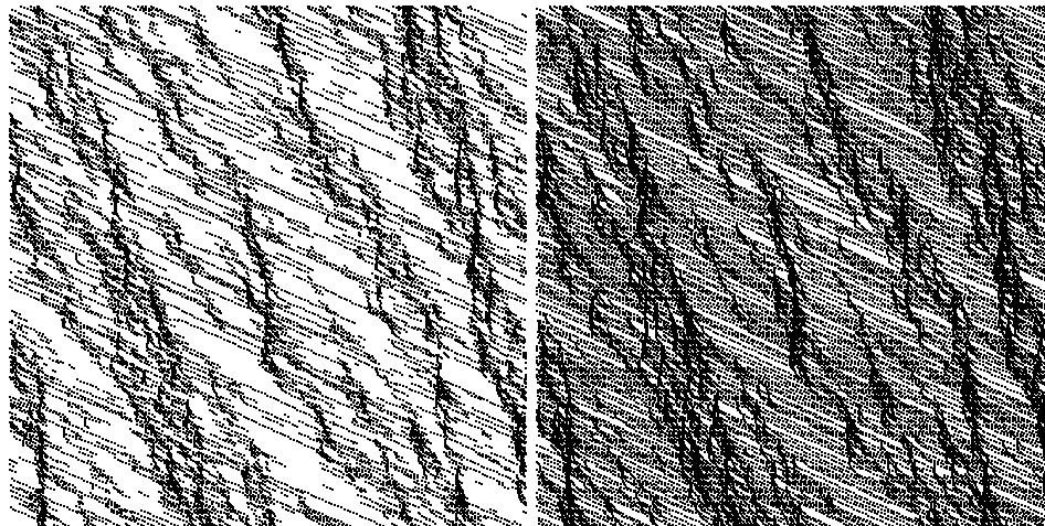
Figure 11: asymmetric, l_{o,back} = 0 , left + right lanes
