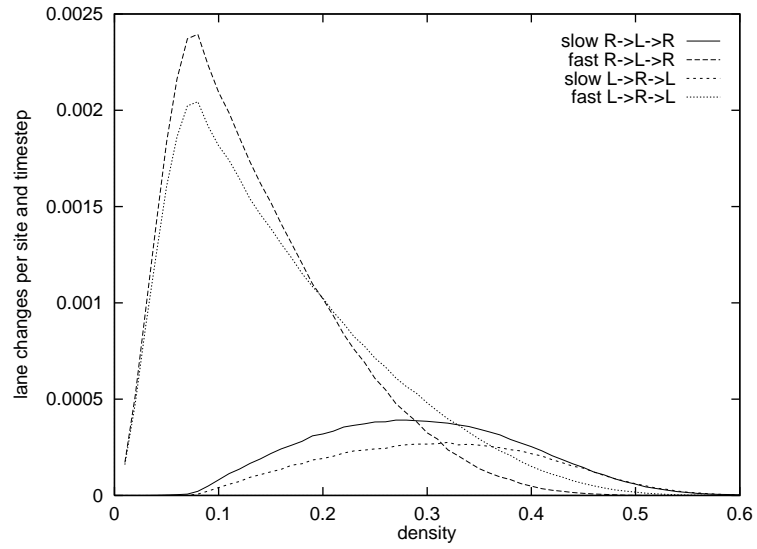
Figure 7: Slow and Fast Ping Pong Lane Changes
