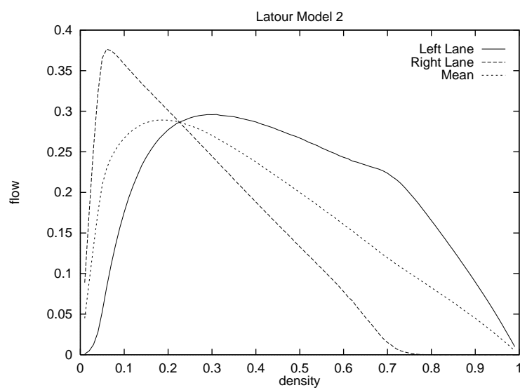
Figure 12: Flow with l = v
