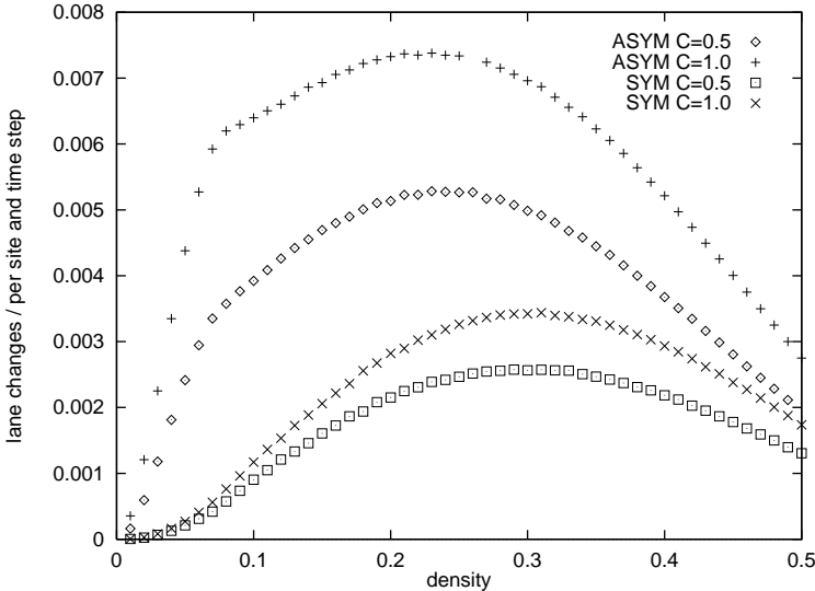
Figure 4: Simple Lane Changes LookBack = 5
