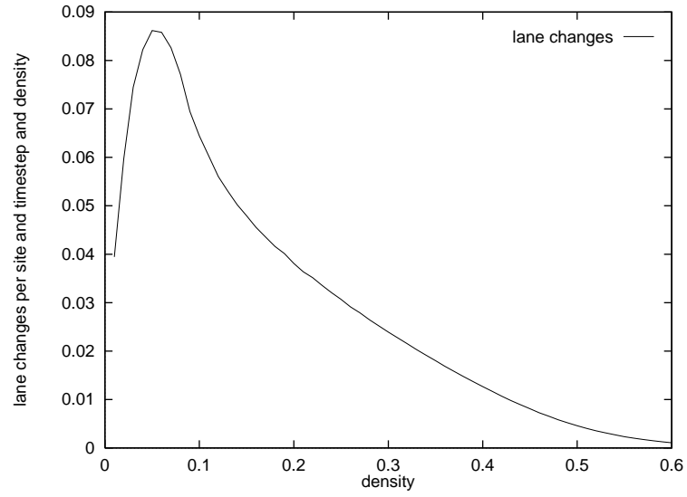
Figure 5: Lane Changes Per Vehicle l = 5 , p_{change} = 1.0
