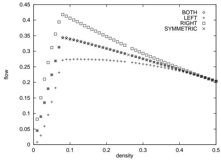
Figure 2: Flow LookBack = 5, p_{change} = 1.0
