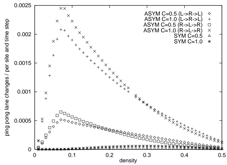
Figure 6: Ping Pong Lane Changes LookBack = 5 , different p_{change}
